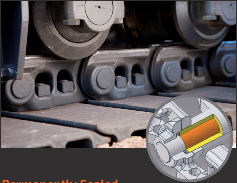
Permanently Sealed, Lubricated Track Pins Pin links on tracked DEVELON material handlers are permanently sealed. They never need greasing. That means you reduce your operating costs and increase your uptime. (DX225MH-5, DX300MH-5)
